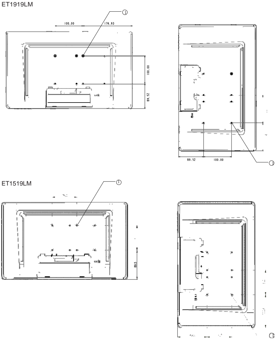
Figure 2-1 : VESA mounting interface location, pedestal removed
