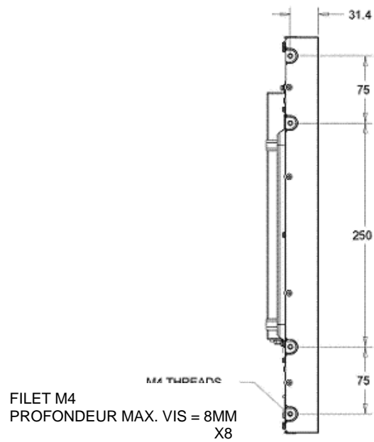
SIDE MOUNT VERITCAL (LEFT/RIGHT) SUPPORT LATÉRAL VERTICAL (GAUCHE/DROITE)
