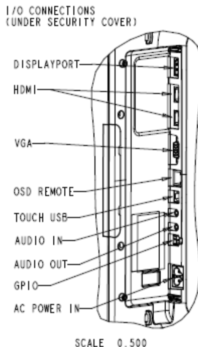
Image of monitors available I/O ports
