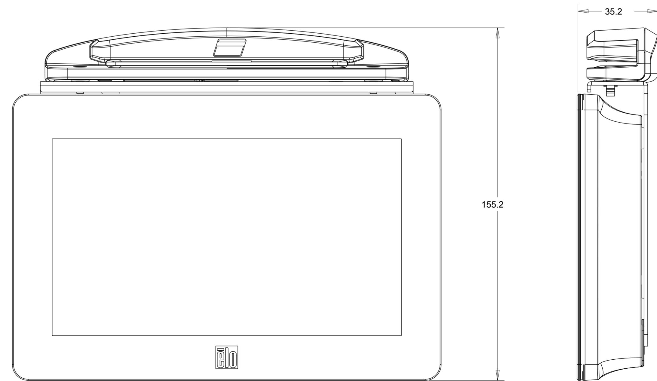
OPTIONAL PERIPHERAL BRACKET (P/N E412148) AND KIT MSR (P/N E039290)
