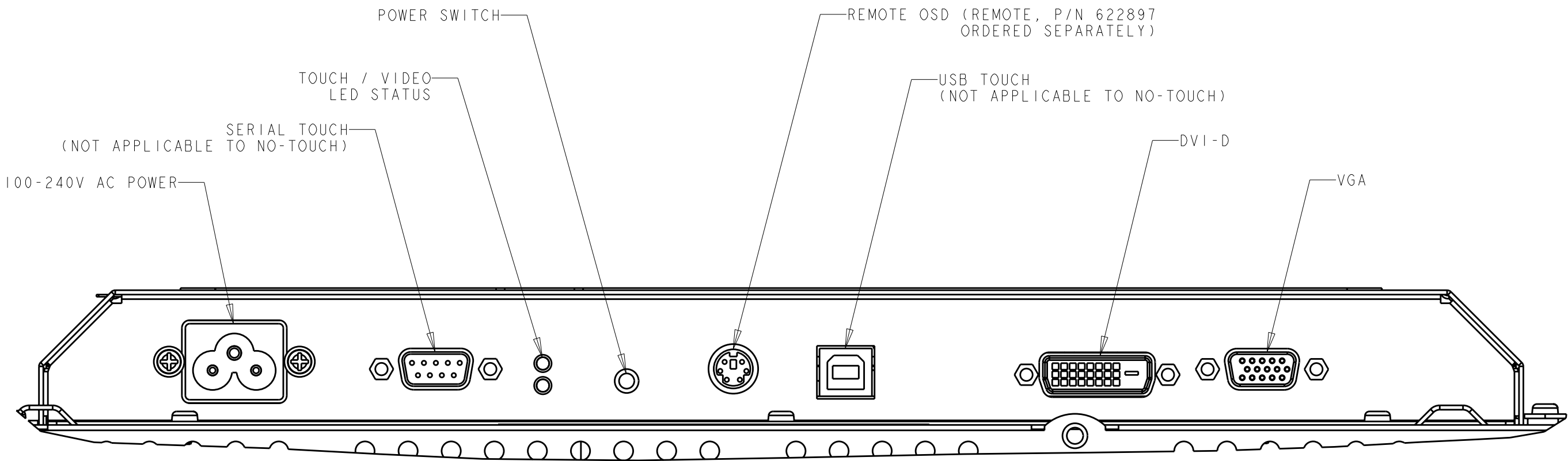
Detail A
