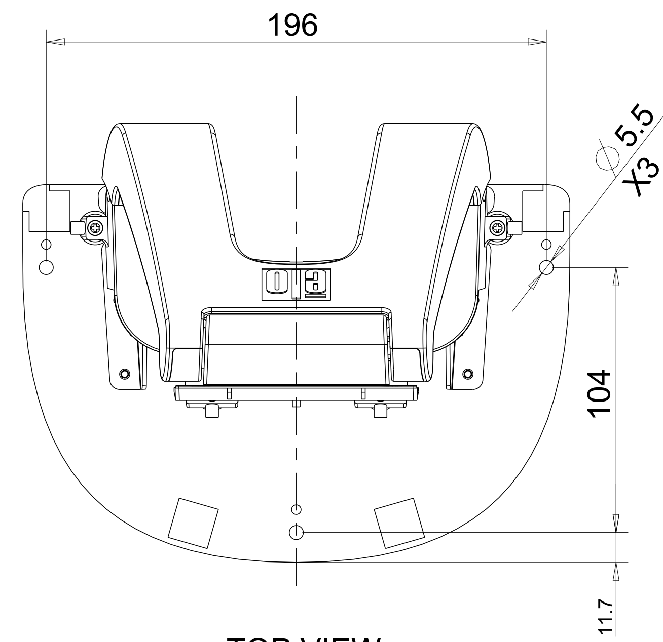
TOP VIEW
