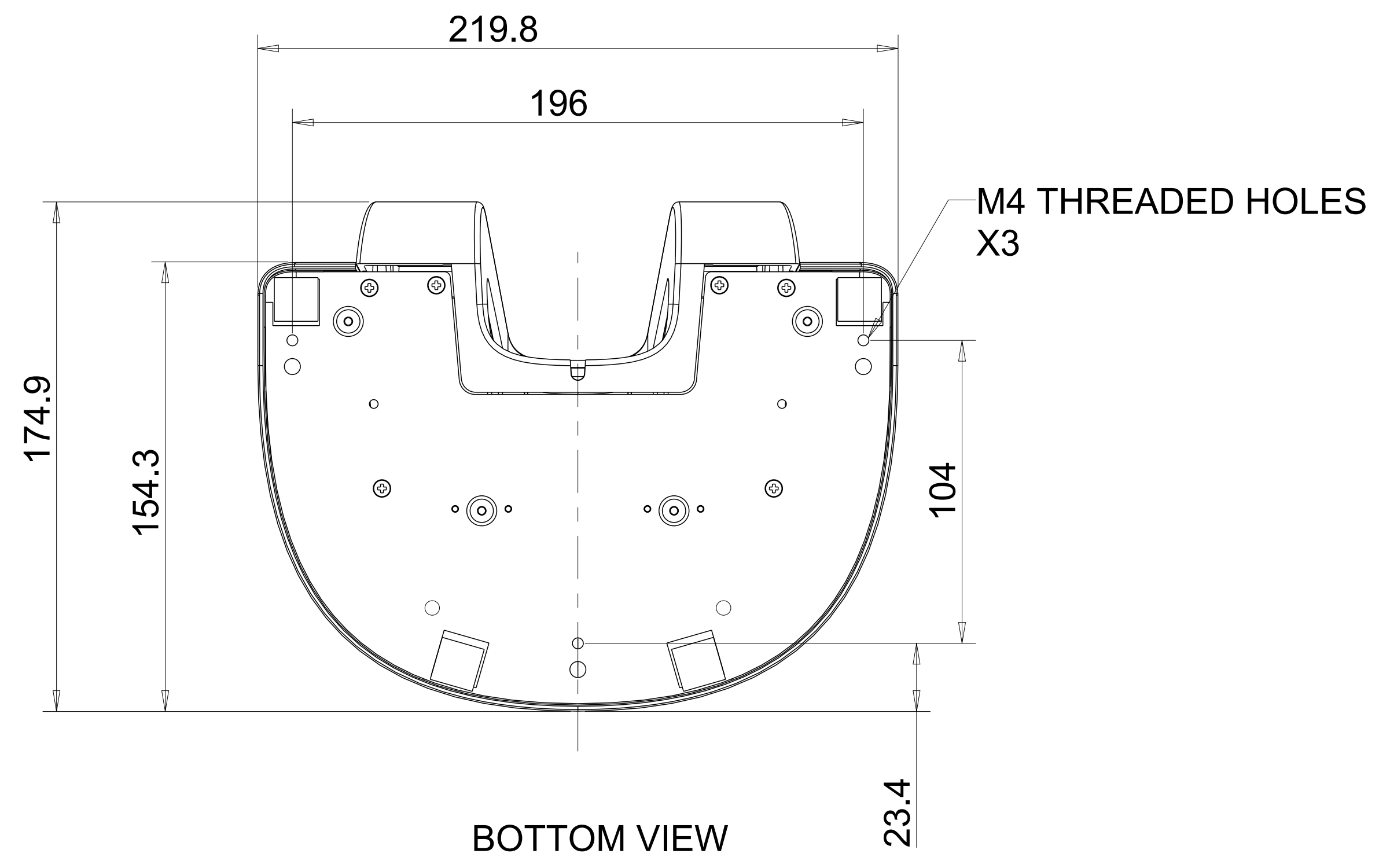
MOUNT OPTION 2
