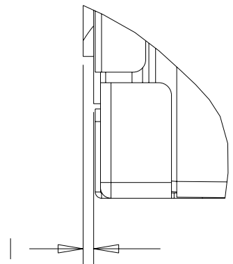
DETAIL A (CENTERING LIP) SCALE 2.000
