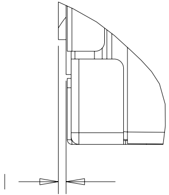
DETAIL A (CENTERING LIP) SCALE 2.000
