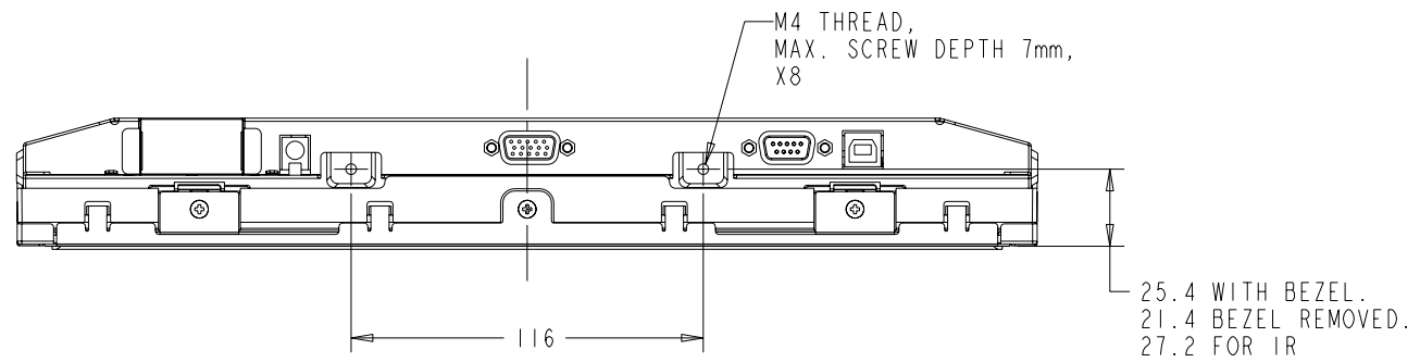
SIDE MOUNT, VERTICAL
