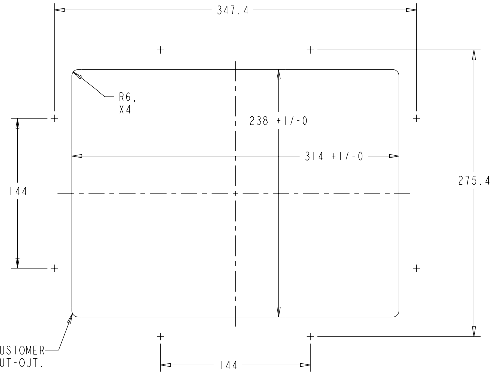
REAR MOUNT, HORIZONTAL AND VERTICAL
