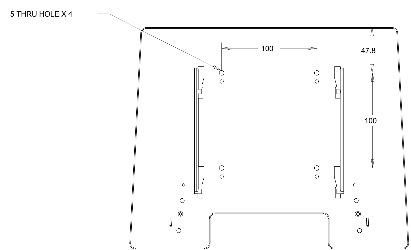
TOP VIEW
