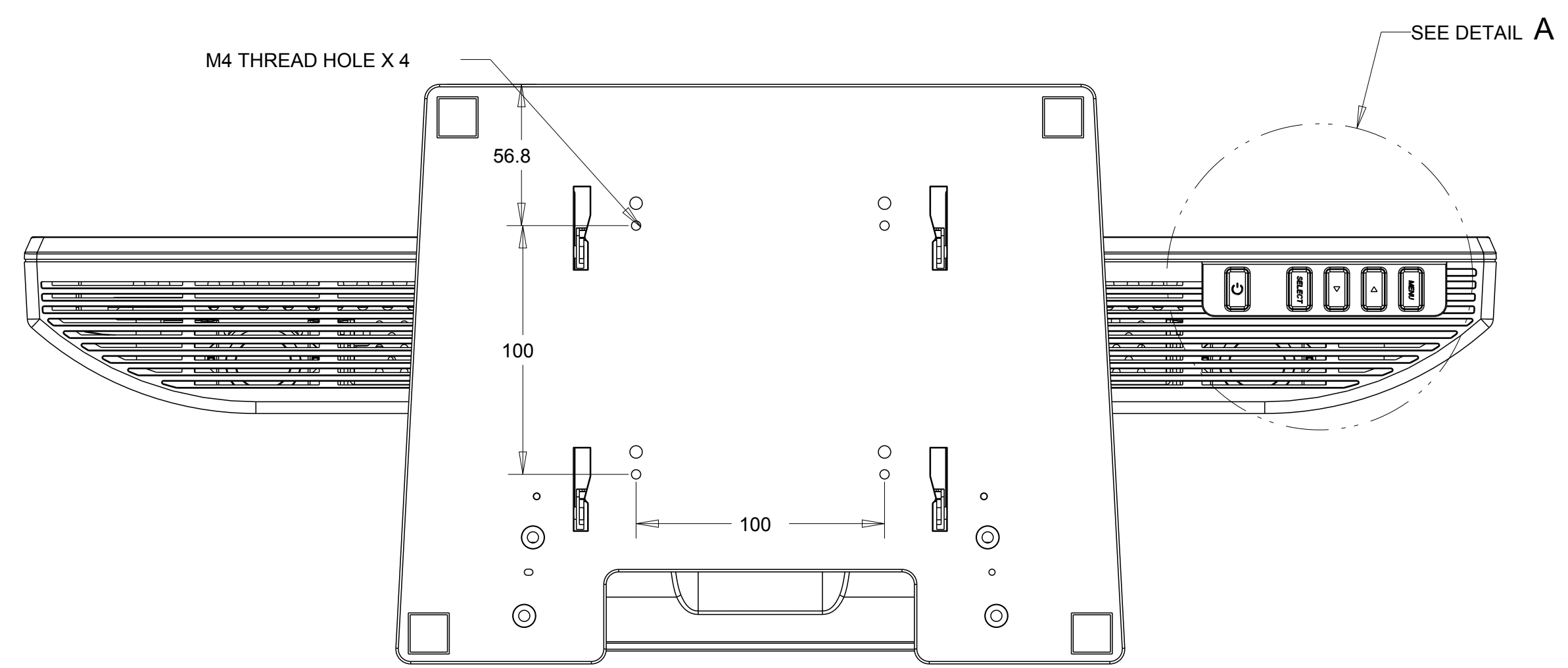
BOTTOM VIEW
