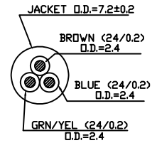
CROSS-SECTION VIEW
