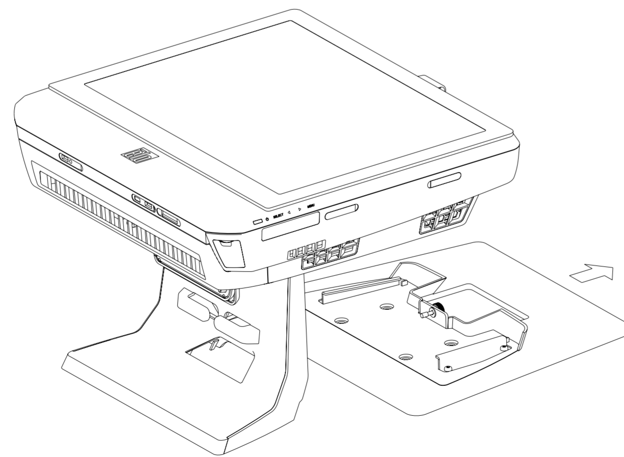
MOUNTING TROUGH HOLES LOCATED ON THE STAND PLATE.
