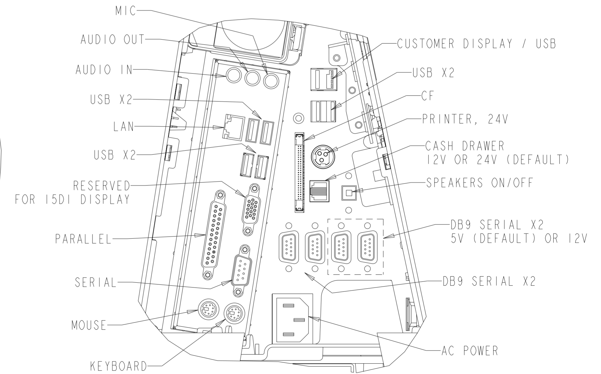
CONNECTOR PANEL
